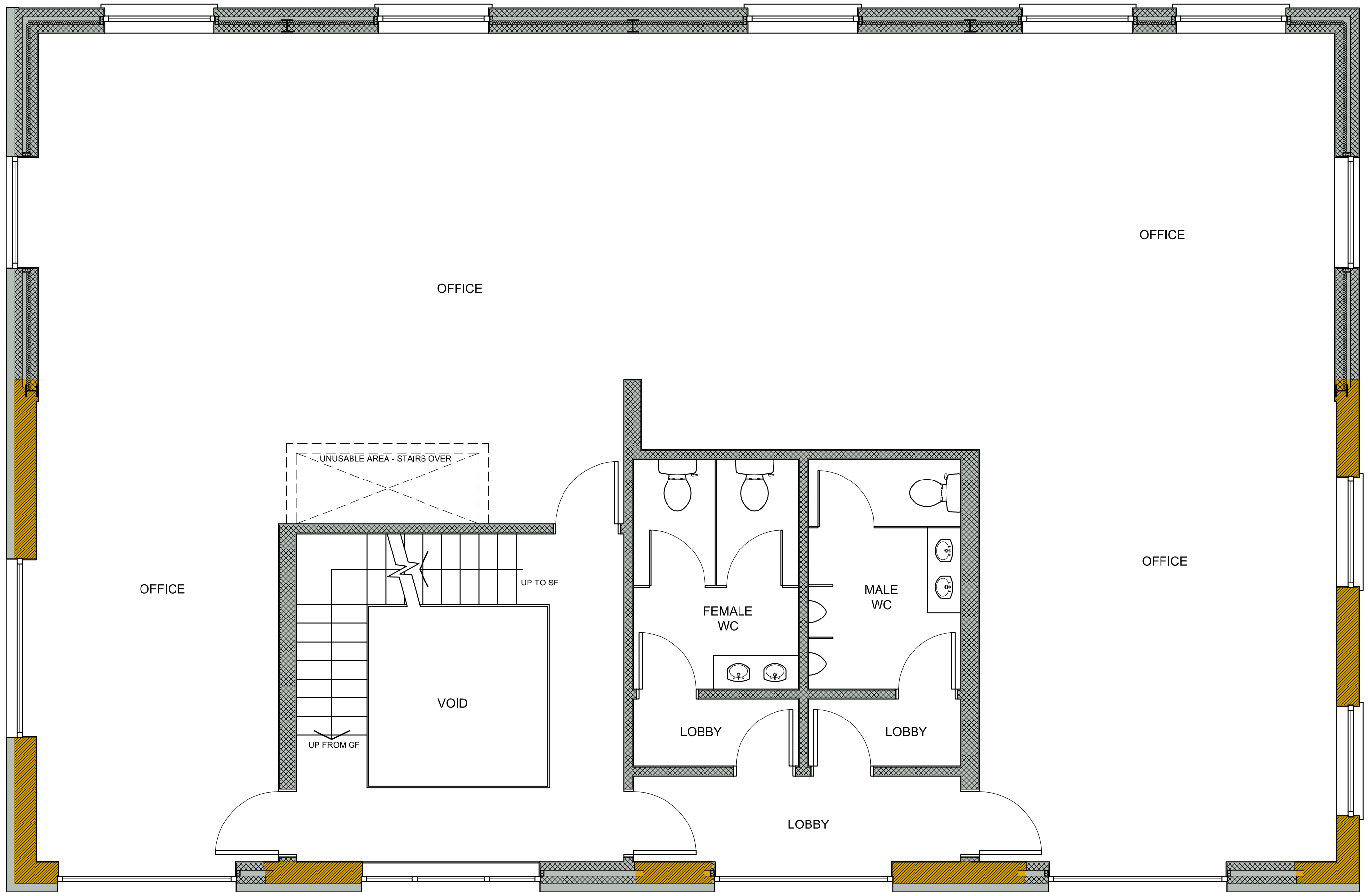
PROPOSED FIRST FLOOR LAYOUT
